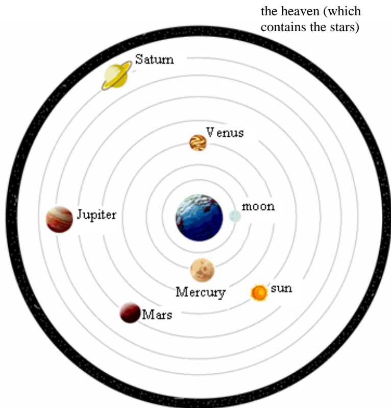
FIGURE 1.2 The Ptolemaic System
