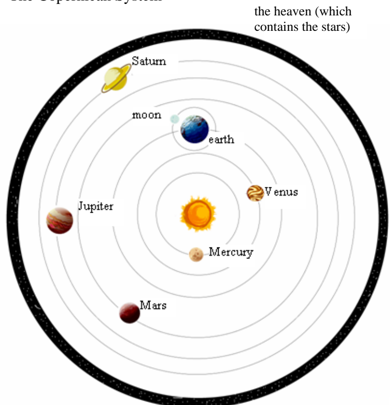
FIGURE 1.4 The Copernican System
