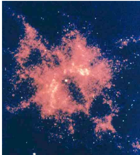
FIGURE 1.3 The Crab Nebula
